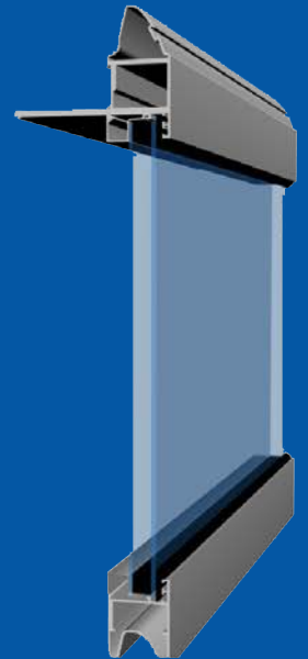
To suit opening width 8000mm Using 100mm profile
